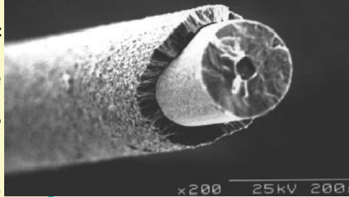
Diamond film on a Textron SiC fibre. The central core is carbon fibre, coated with SiC and then 22µm of CVD diamond.
